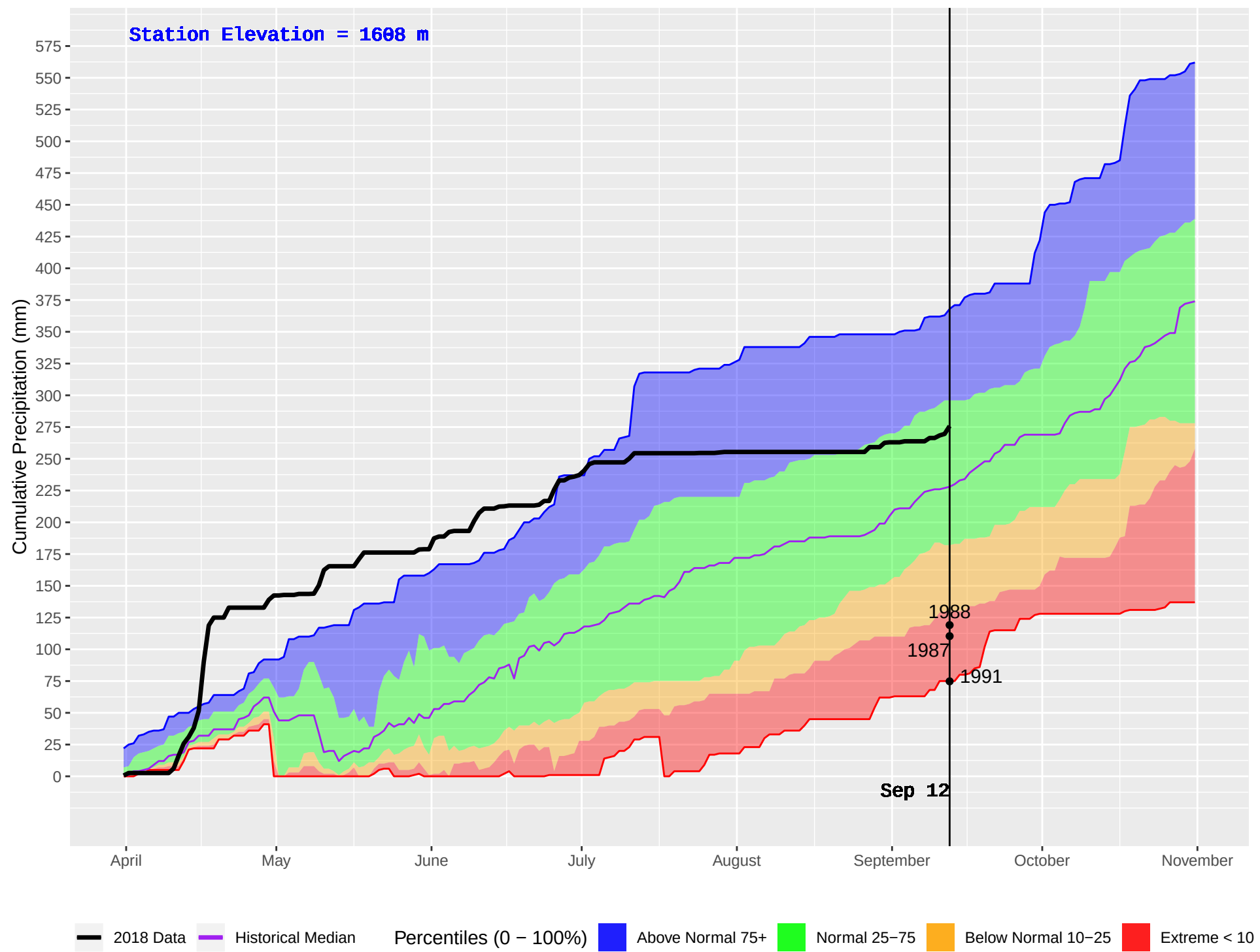
DEWAR CREEK (421) : Historical (1986–2016) and Current (2018) Daily Cumulative Precipitation
