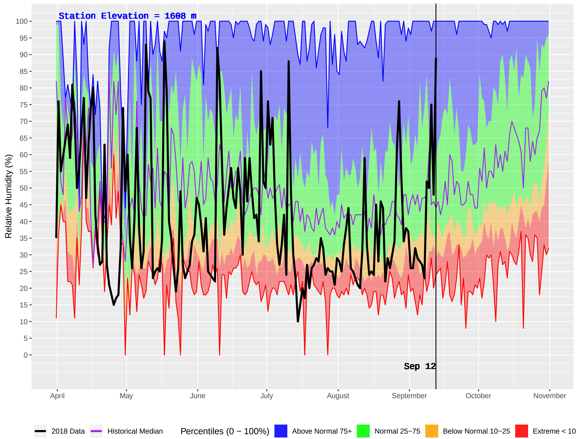
DEWAR CREEK (421) : Historical (1986–2016) and Current (2018) Daily Relative Humidity
