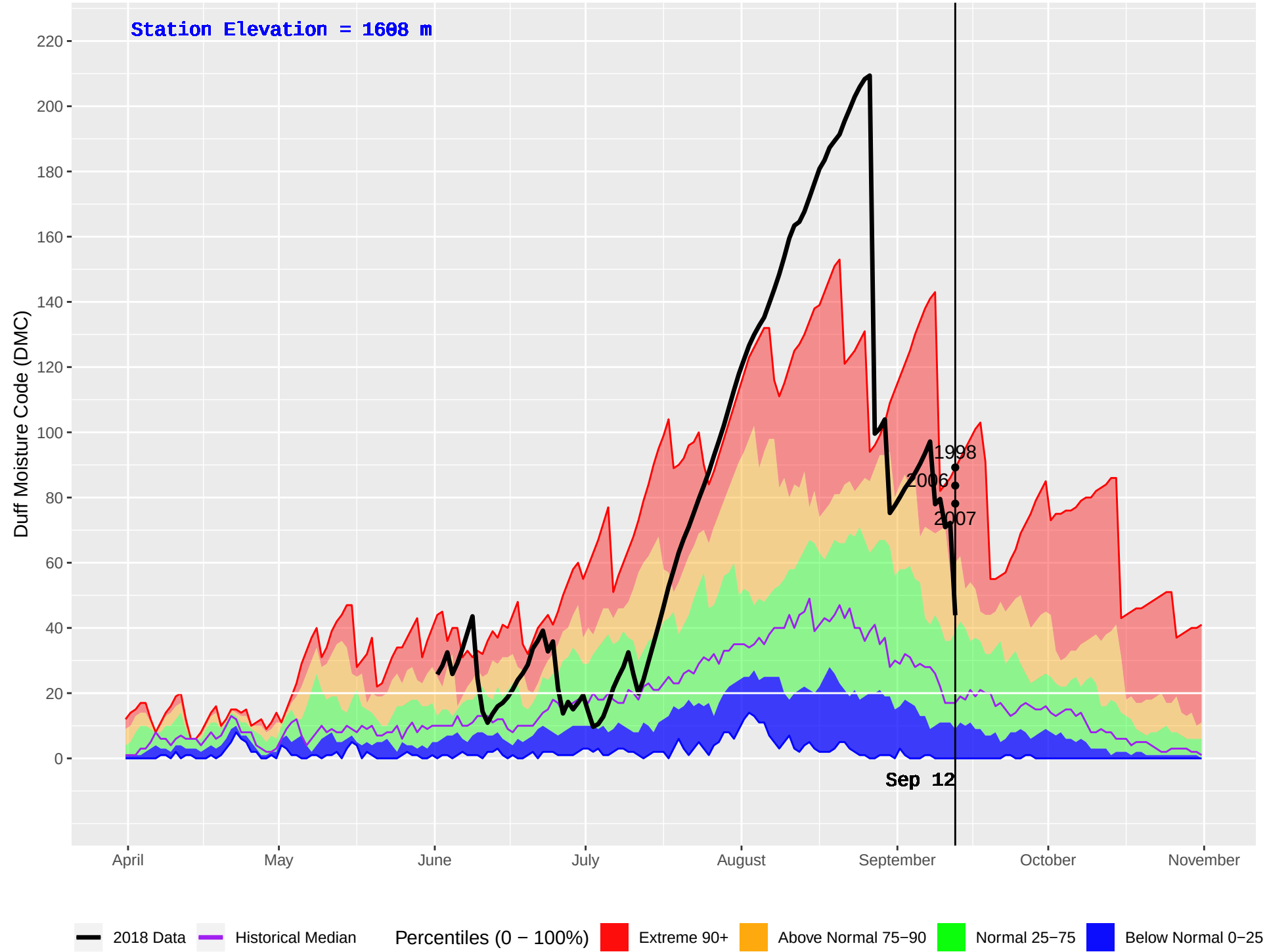
DEWAR CREEK (421) : Historical (1986–2016) and Current (2018) Daily Duff Moisture Code (DMC)
